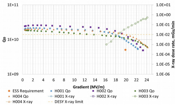
Figure 3: H001 - H004 dressed cavity testing at DESY
