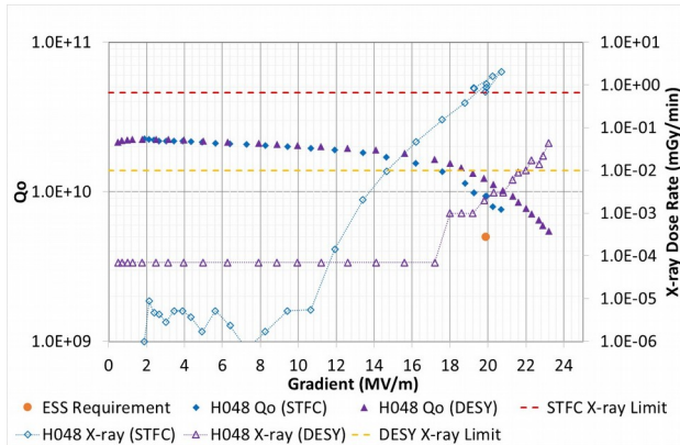
Figure 7: Radiation comparison of H048 at STFC and DESY
